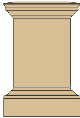
Bampfylde Pedestal (UP24) Height 982mm Base Width 654mm Shaft Width 490mm Cap Width 654mm Cap top width 460mm
