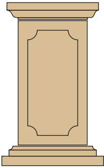
French Pedestal (UP08) Height 850mm Base Width 533mm Shaft Width 362mm Cap Width 480mm
