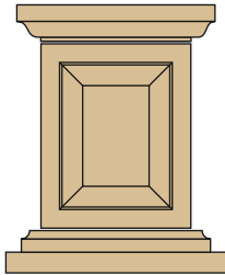
Panelled Pedestal (UP04) Height 647mm Base Width 533mm Shaft Width 365mm Cap Width 480mm
