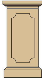
Classical Pedestal (UP05) Height 676mm Base Width 332mm Shaft Width 280mm Cap Width 365mm
