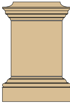
Popes Pedestal (UP23) Height 847mm Base Width 582mm Shaft Width 435mm Cap Width 582mm Cap top width 400mm
