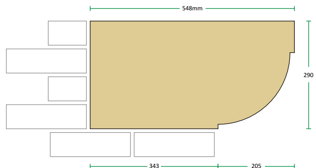
CB3 Corbel
