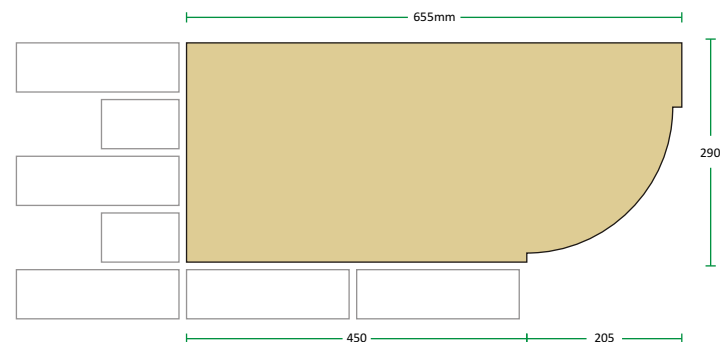
CB4 Corbel
