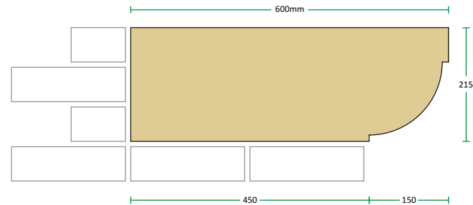
CB2 Corbel
