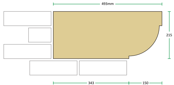
CB1 Corbel
